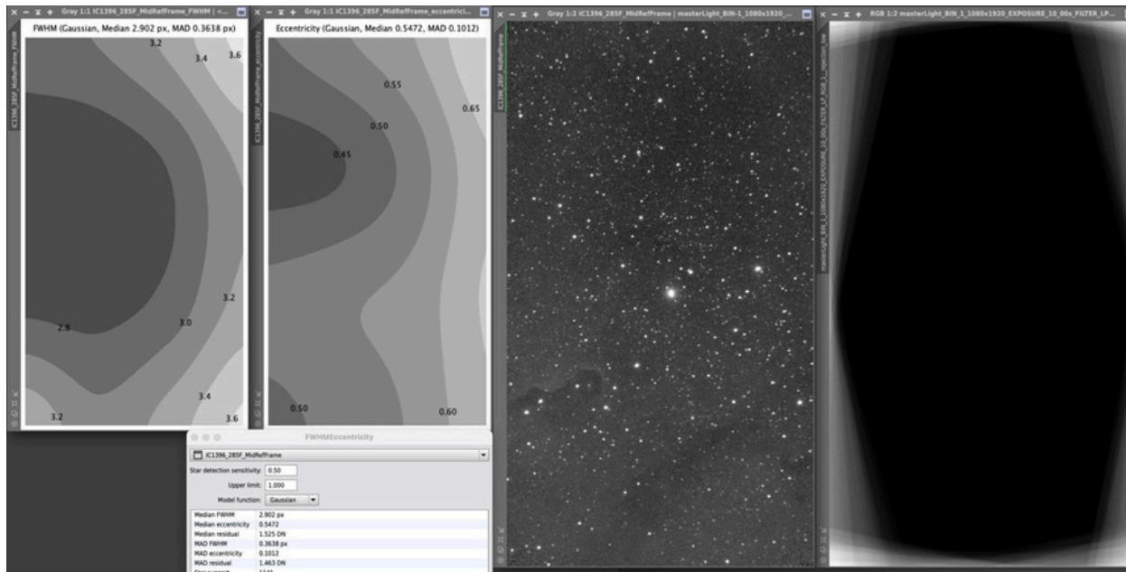
Figure 25 - It can be clearly seen how the alignment of the stacking has been improved by selection of a central reference frame.
